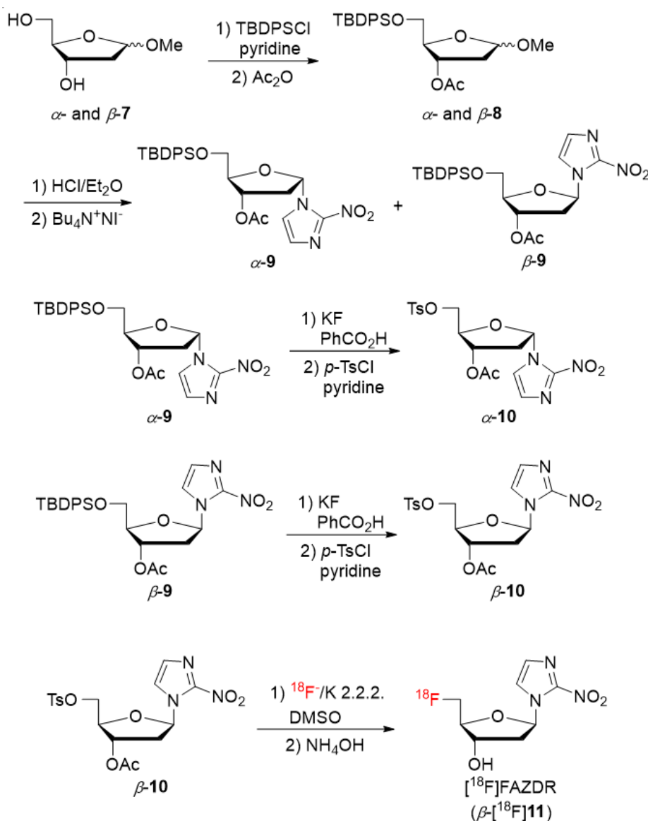
Fig. 2. Synthesis of the precursors \alpha -9 and \beta -9 and radiosynthesis of [ ^{18}\text{F} ]FAZDR ([ ^{18}\text{F} ]- \beta -11).
