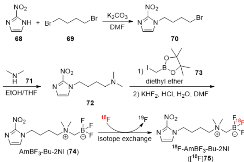
Fig. 9. Synthesis and radiofluorination precursor \text{AmBF}_3 - Bu - 2NI.
