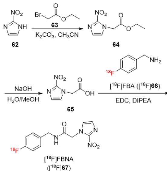
Fig. 8. Synthetic of ^{18}\text{F} -labeled radiotracer [^{18}\text{F}]\text{FBNA} .
