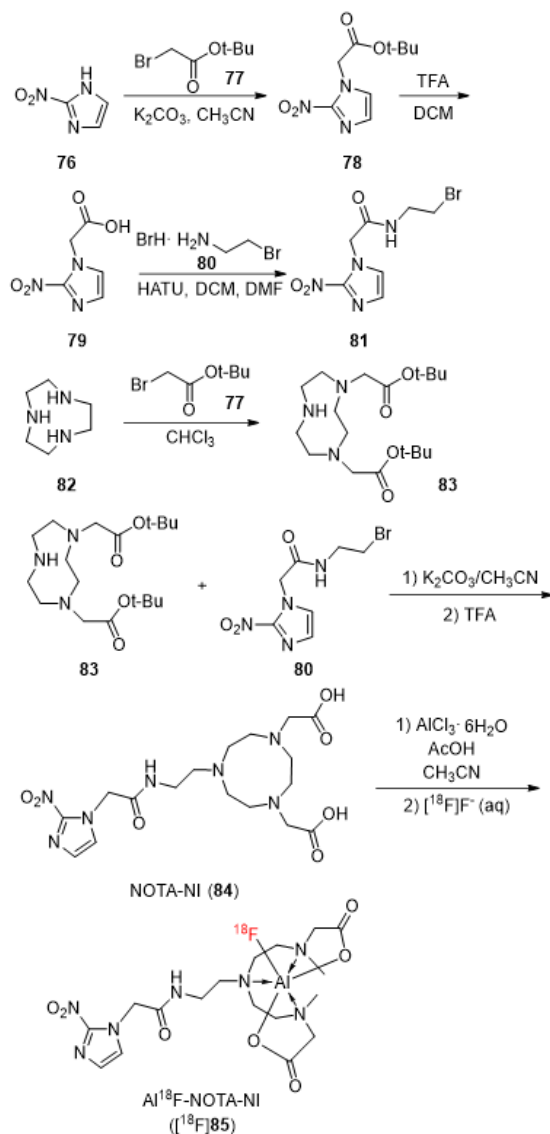
Fig. 10. Synthetic route to precursor NOTA-NI and radiosynthesis of radiotracer \text{Al}^{18}\text{F} -NOTA-NI
