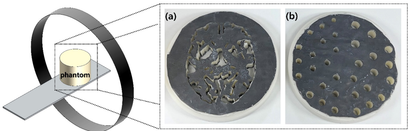
Fig. 1. The This photo is PET scanner and dedicated PET phantom images using the 3D printing technology by adding lead material with (a) Hoffman and (b) Derenzo phantom.
